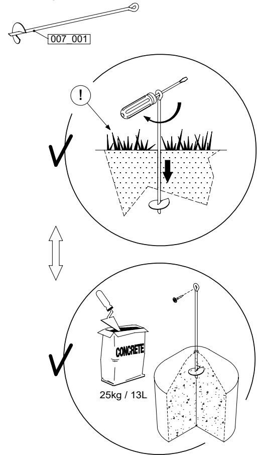
Screw-in ground anchor
