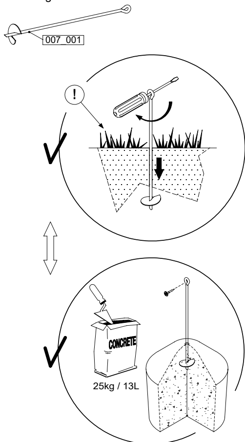
Screw-in ground anchor
