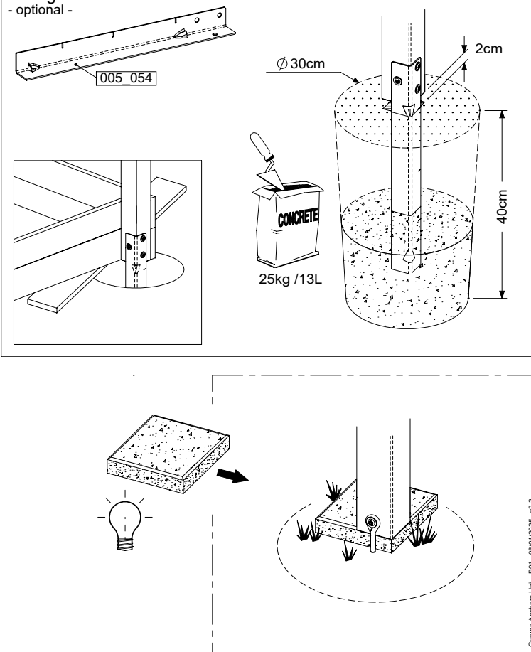
Post ground anchor - optional -
