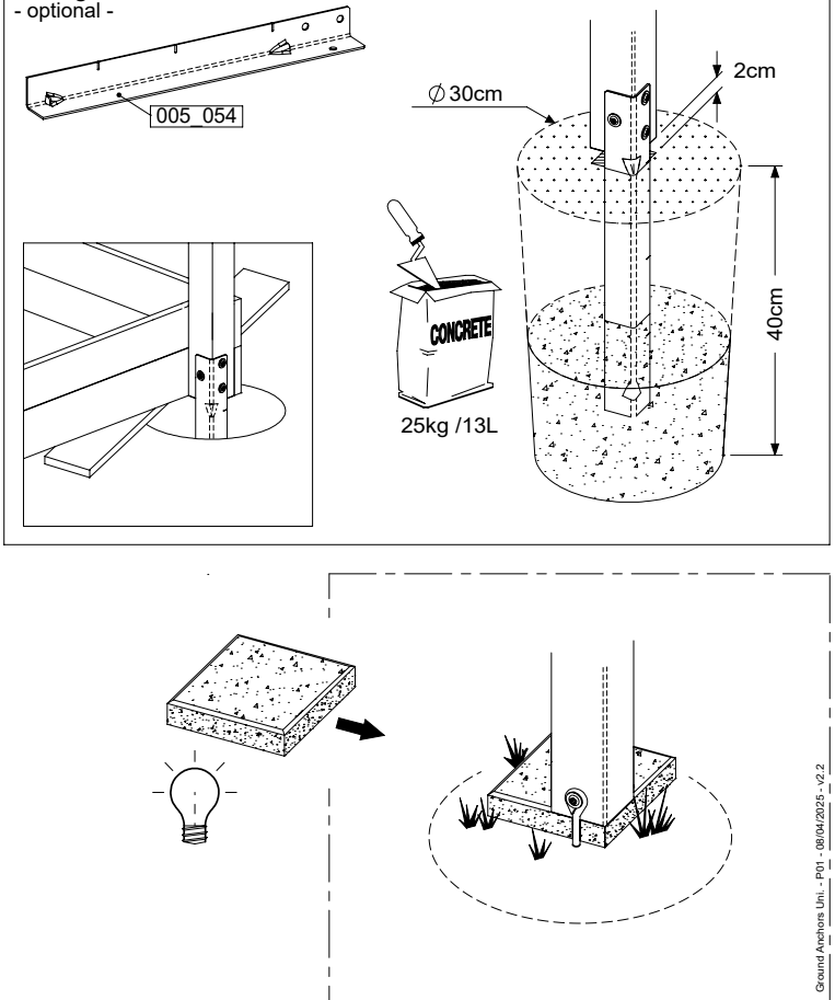
Post ground anchor - optional -
